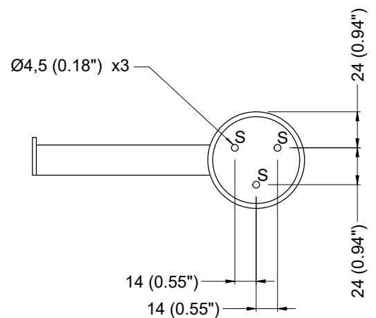
BACK VIEW WALL MOUNTING
