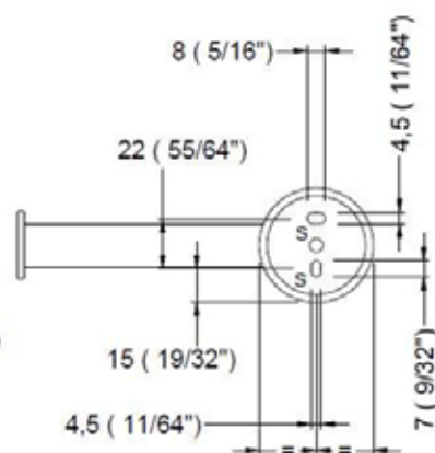
BACK VIEW WALL MOUNTING
