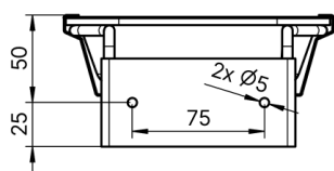
Bohrbild | drilling pattern
