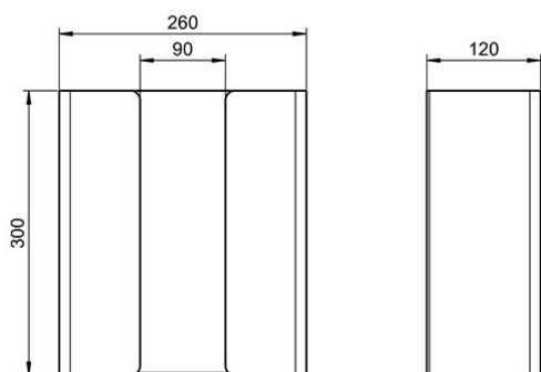
Bohrbild | drilling pattern
