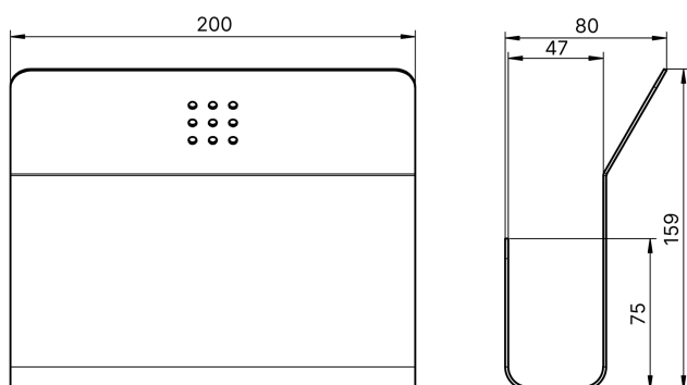
Bohrbild | drilling pattern
