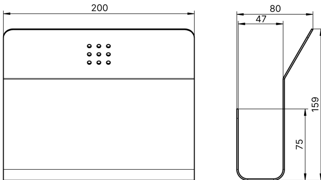
Bohrbild | drilling pattern
