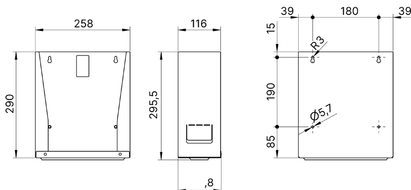
Bohrbild | drilling pattern
