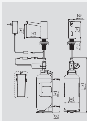
MATRIX PRIMUS SEIFENSPENDER, BATTERY 1991810
