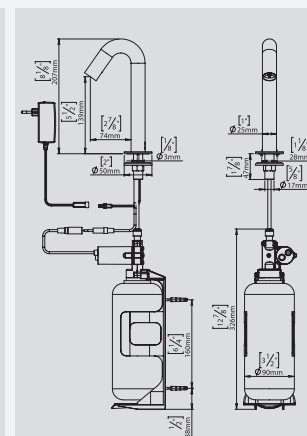
SINTRA SEIFENSPENDER, BATTERY 1991210
