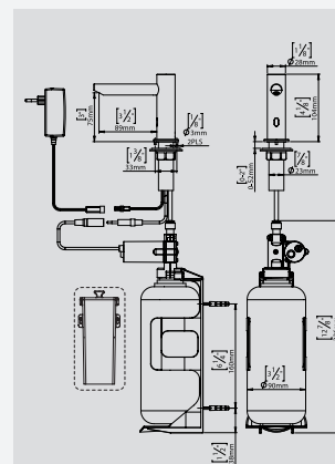
MATRIX SEIFENSPENDER, BATTERY 1991010
