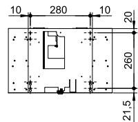
Bohrbild | drilling pattern
