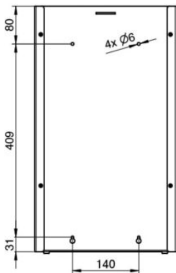
Bohrbild | drilling pattern
