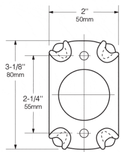
Endmontageflansch
