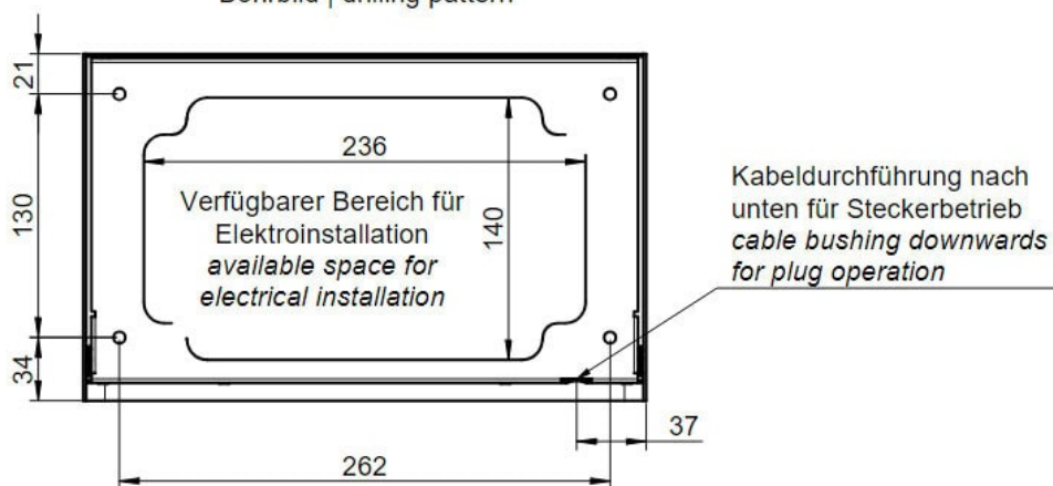
Bohrbild | drilling pattern
