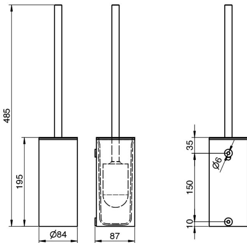
Bohrbild | drilling pattern
