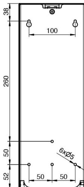
Bohrbild I drilling pattern
