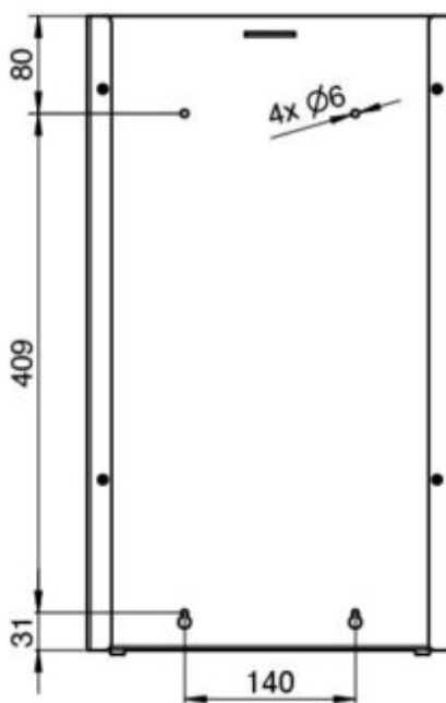
Bohrbild | drilling pattern
