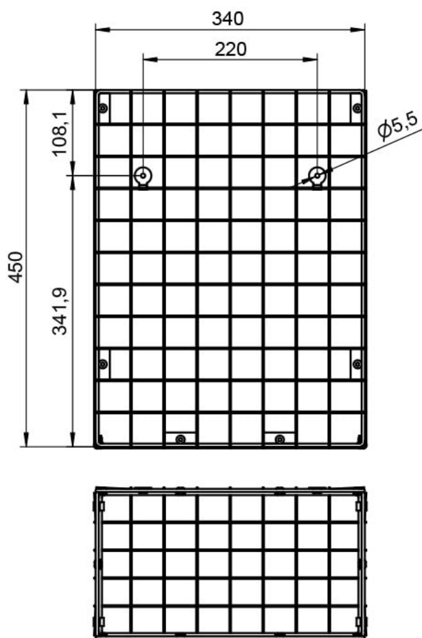
Bohrbild | drilling pattern
