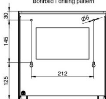
Bohrbild | drilling pattern
