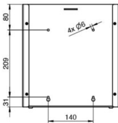
Bohrbild | drilling pattern
