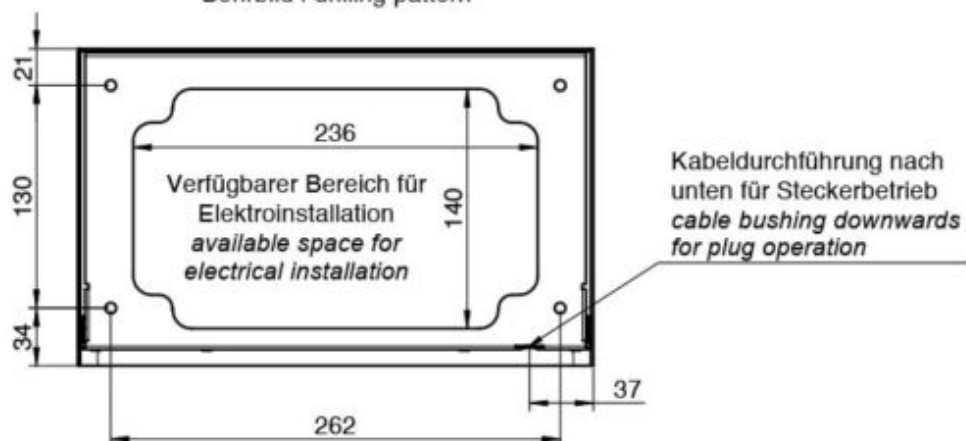
Bohrbild | drilling pattern
