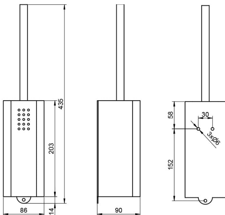
Bohrbild | drilling pattern
