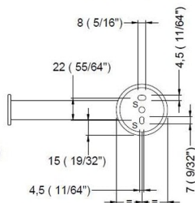
BACK VIEW WALL MOUNTING
