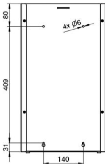
Bohrbild I drilling pattern
