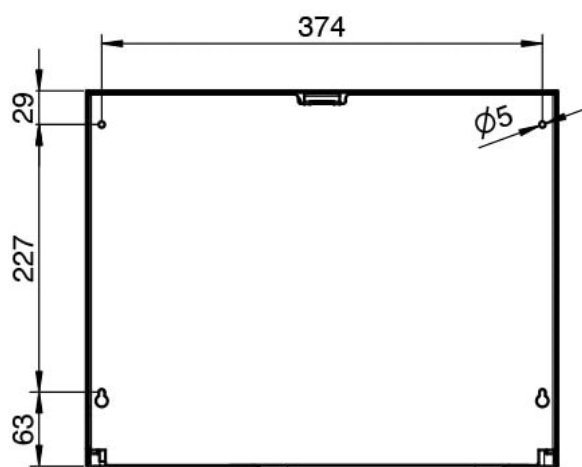
Bohrbild | drilling pattern
