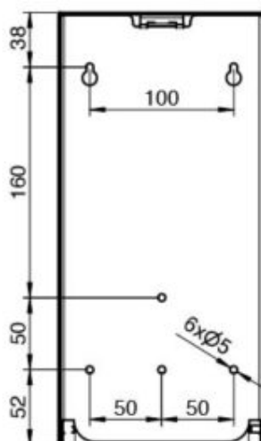
Bohrbild | drilling pattern
