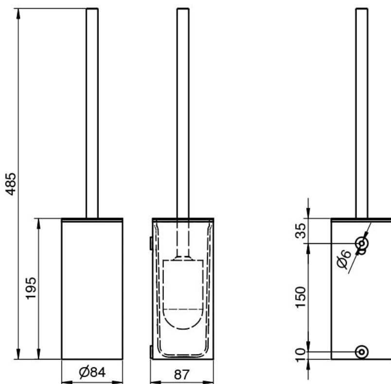
Bohrbild I drilling pattern
