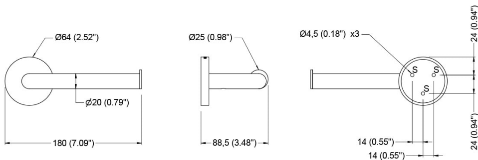
BACK VIEW WALL MOUNTING
