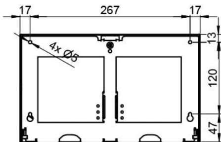
Bohrbild | drilling pattern
