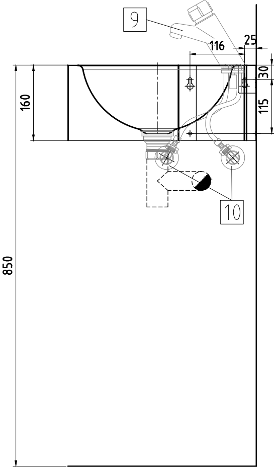
Drain valve assembly 1 1/4"
