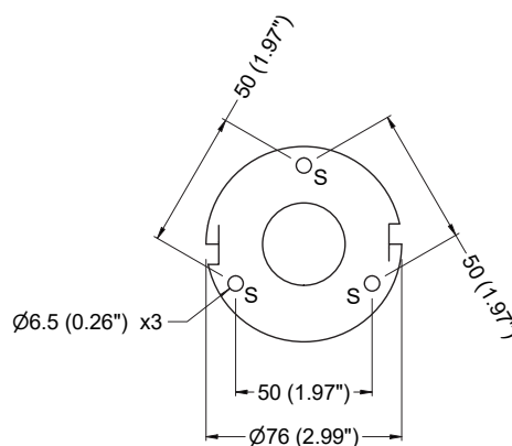
BACK VIEW WALL MOUNTING
