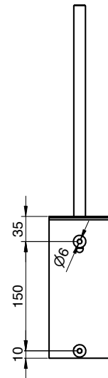
Bohrbild | drilling pattern
